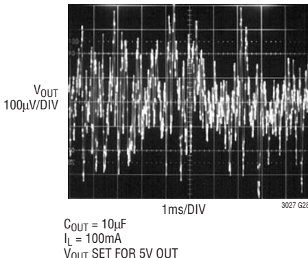
10Hz to 100kHz Output Noise C_{\text{BYP}} = 0
